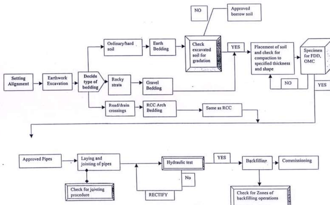
Figure 8.2 PROCESS CHART FOR PIPELINE WORKS WITH STAGES OF INSPECTION
